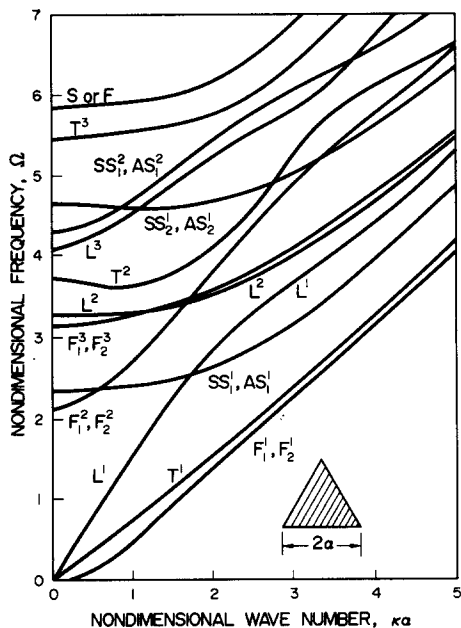
Fig. 13. First thirteen branches of the complete spectra for an equilateral triangle waveguide (Poisson's ratio \nu = 1/3 , 45 element half-bar model).
